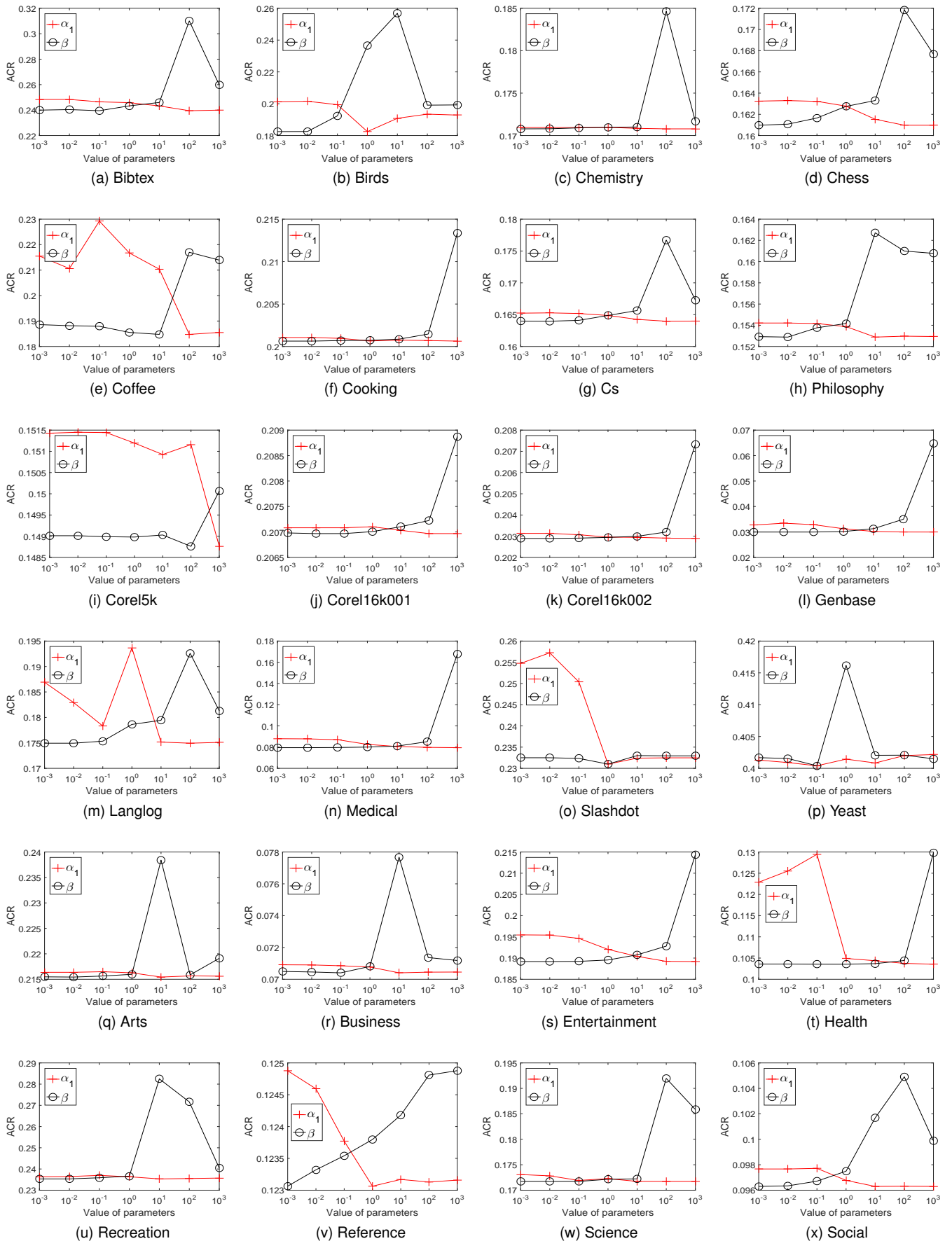
Fig. 1. Parameter analysis of GRRO on the 24 data sets.
